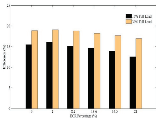
Fig. 16. Variation of brake thermal efficiency for different EGR flow rates at part loads
